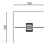
Arch 2 Places L.120cm W.120cm H.72cm Séparation: H.35 cm
